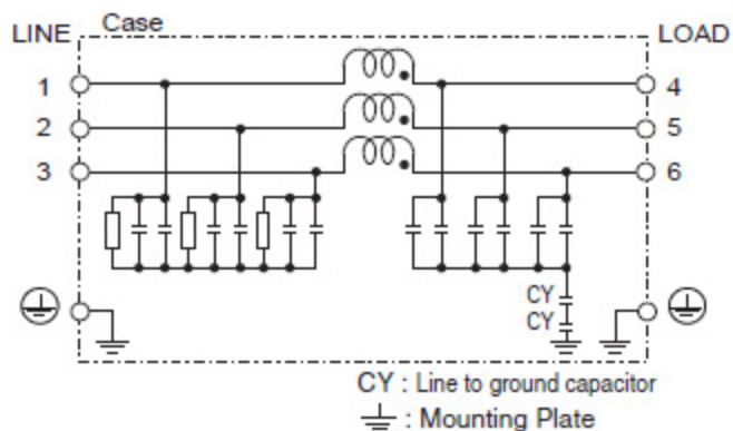
(4) Line to ground capacitor code : 155, 335 Option : U
