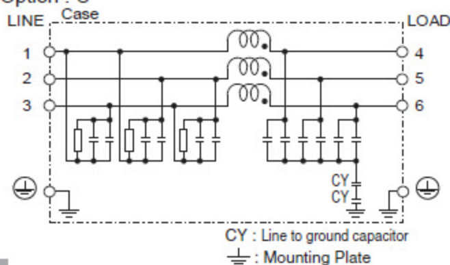
(3) Line to ground capacitor code : 223, 683, 104 Option : U
