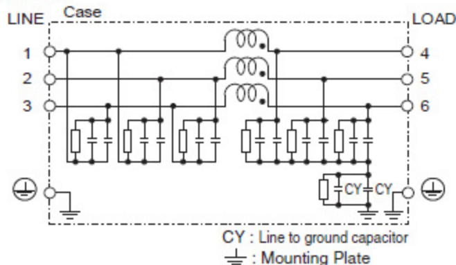
(4) Line to ground capacitor code : 155, 335 Option : U
