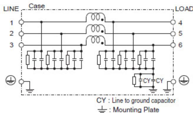
(5) Line to ground capacitor code : 155, 335 Option : G
