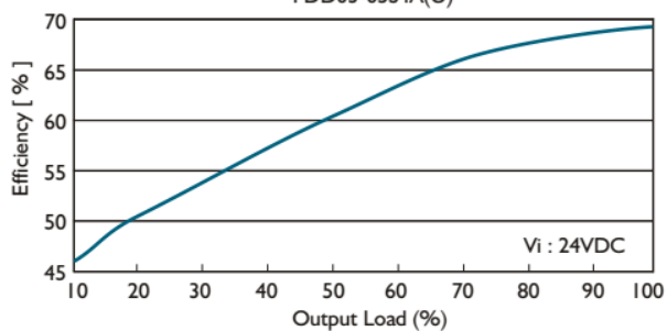
Efficiency Vs Output Load FDD03-05S4A(U)
