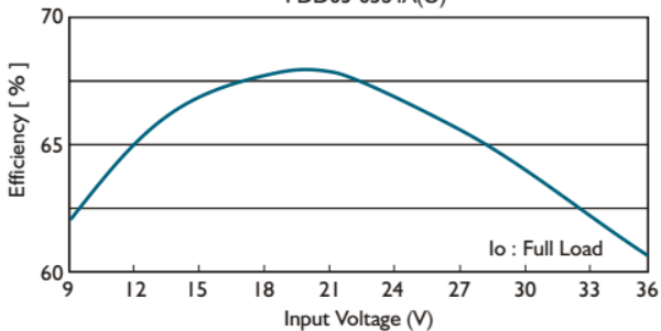
Efficiency Vs Input Voltage FDD03-05S4A(U)
