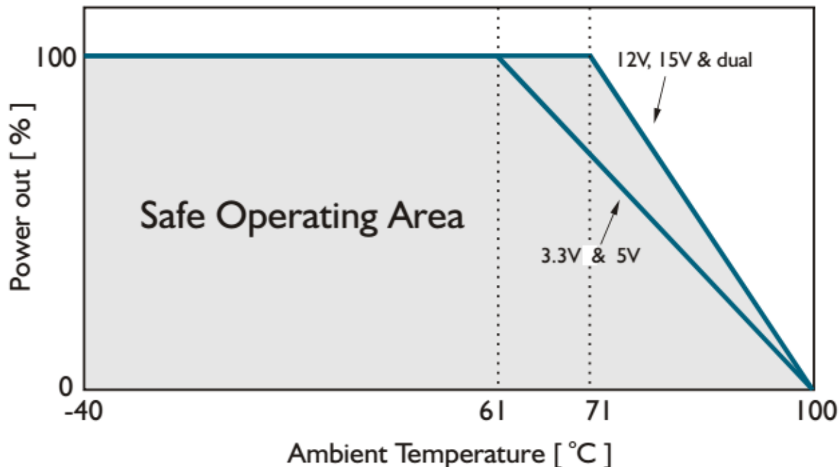
Temperature derating curve
